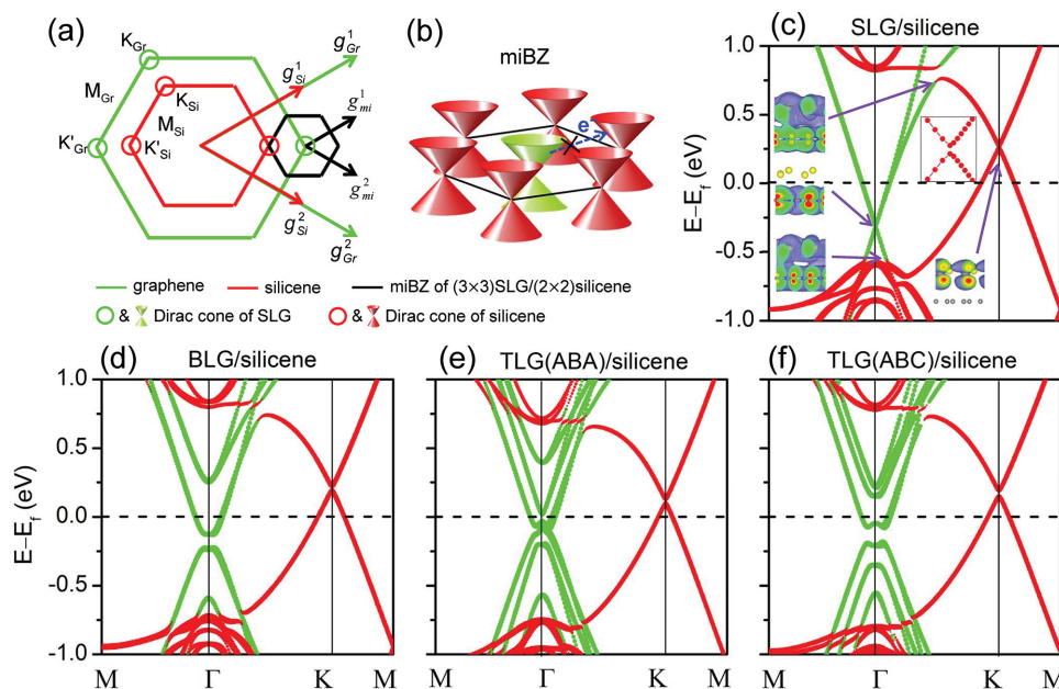
Figure 2. a) Brillouin zones (BZs) of the silicene and graphene lattices drawn to scale. Mini BZ (miBZ) of the (3 \times 3)\text{SLG}/(2 \times 2)\text{silicene} heterostructure is indicated around the K point of graphene ( K_{\text{Gr}} ). b) Dirac cones of graphene (green) and silicene (red) in the miBZ. c–f) Band structures of the SLG, BLG, ABA- and ABC-stacked TLG/silicene heterostructures. Silicene-dominated bands (red) are plotted against the graphene projected bands (green). The wave functions at four (k, E) points are represented in the insets of c), with an isovalue of 0.002 \text{ e}/\text{\AA}^3 .
