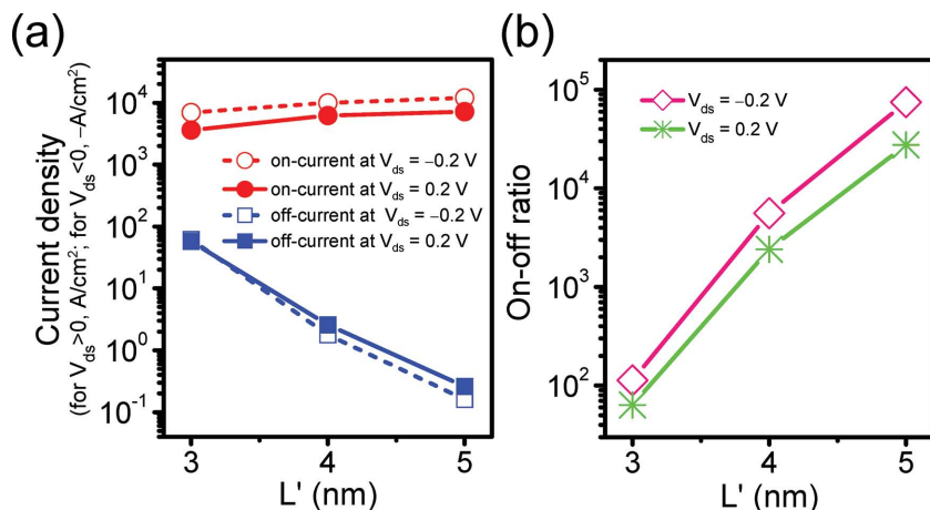
Figure 4. a) On- and off-current densities and b) on/off current ratio under V_{ds} = -0.2 and 0.2 V in the local-gated (3 \times 3) SLG/ (2 \times 2) silicene heterostructure device with L' = 3, 4 , and 5 nm, respectively. The gate voltage range is -5 \sim 5 V.
